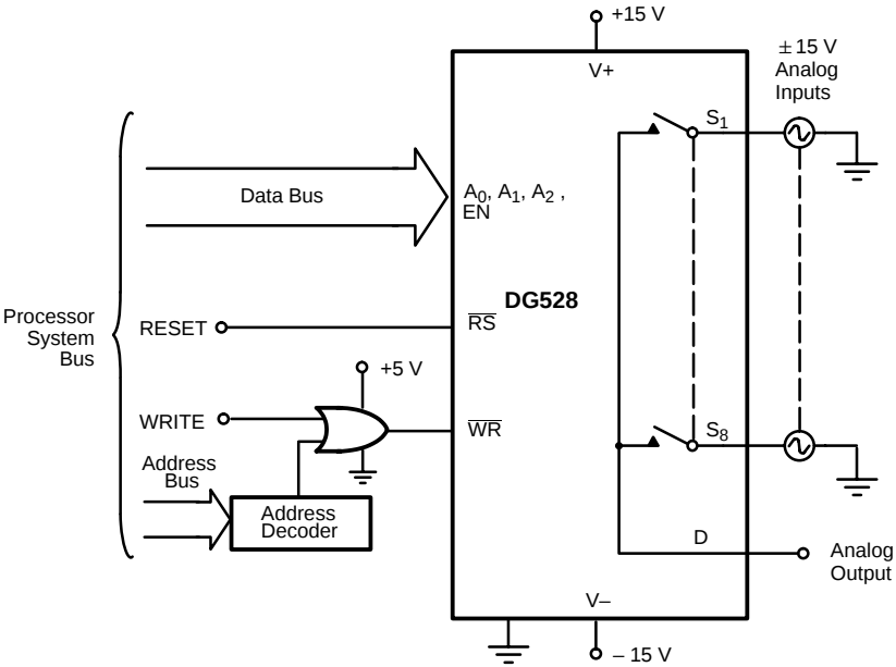
FIGURE 9. Bus Interface
