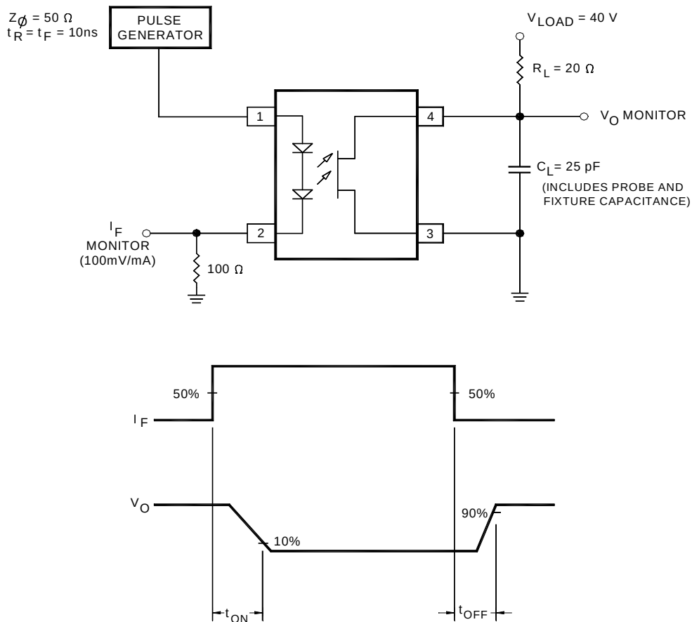
Figure 3. Switching Waveforms and Test Circuits
