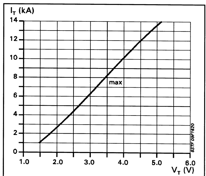
Fig.3 On-state characteristics.
