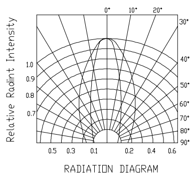
Radiation Diagram T_a=25^\circ
