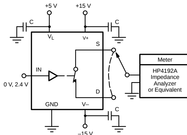
FIGURE 7. Source/Drain Capacitances
