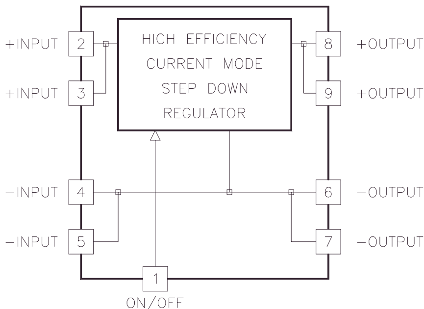
11-17 Watt SD Single Series Block Diagram
