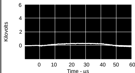
FIGURE 2 TYPICAL CLAMPING ACTION OF A 16 AMP MODULE
