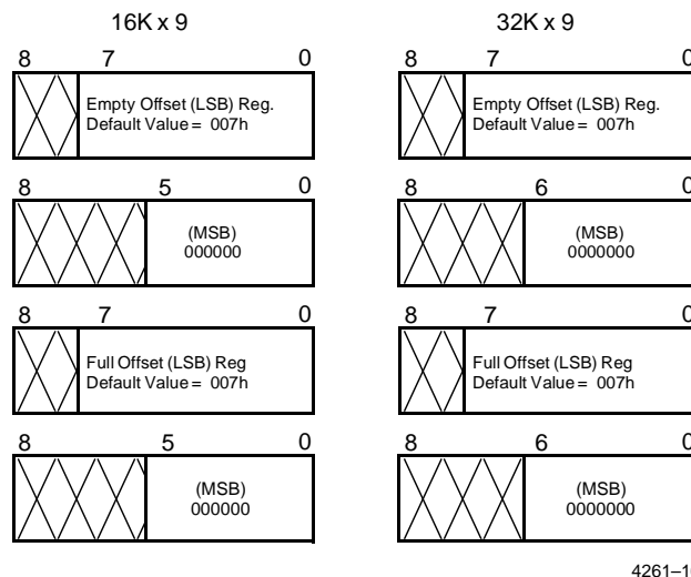
4261-16 Figure 1. Offset Register Location and Default Values
