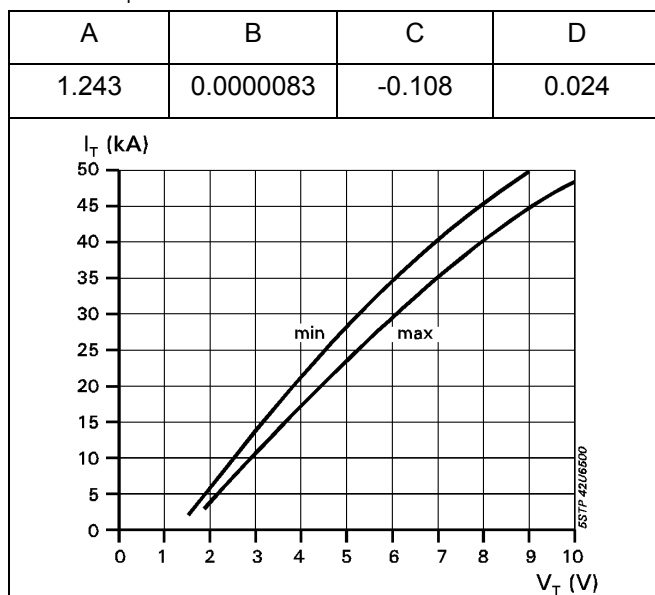
Fig. 2 On-state characteristics. T_j=125^\circ\text{C} , 10ms half sine
