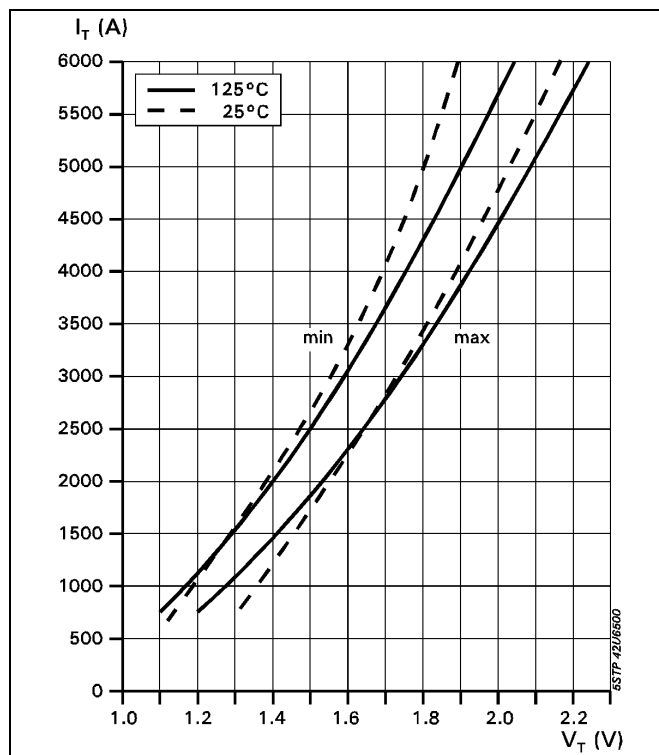
Fig. 3 On-state characteristics.
