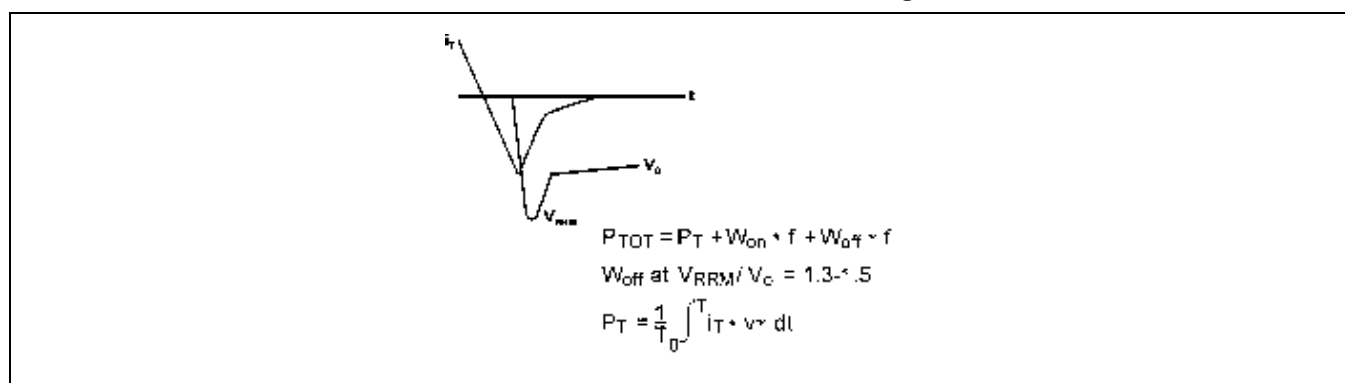
Fig. 17 W_{off} = f(V_0, I_T) , T_j = 125^\circ\text{C} . Half sinusoidal waves. t_p = 10 ms.
