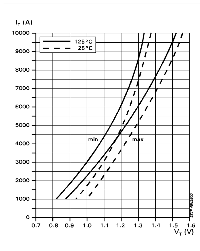
Fig. 3 On-state characteristics.
