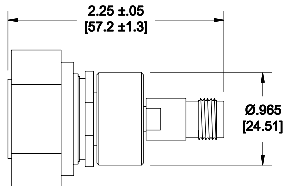
Model Number: 5710 7/16 - DIN Male / TNC Female
