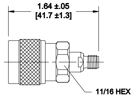
Model Number: 5147 Type N Female / 3.5mm Female
