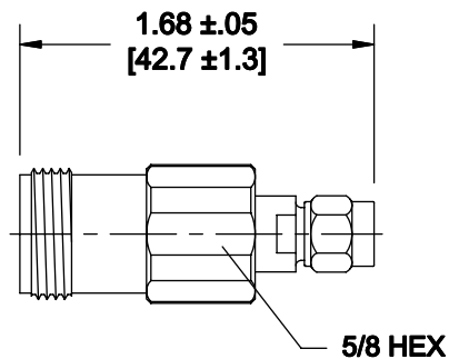
Model Number: 5146 Type N Female / 3.5mm Male
