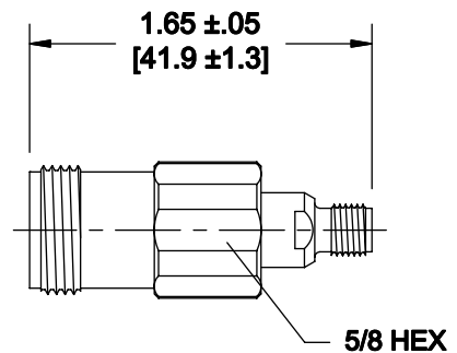
Model Number: 5147 Type N Female / 3.5mm Female
