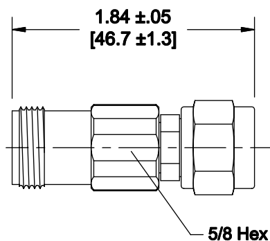
Model Number: 5128 Type N Female / TNC Male
