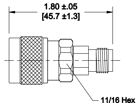
Model Number: 5127 Type N Male / TNC Female
