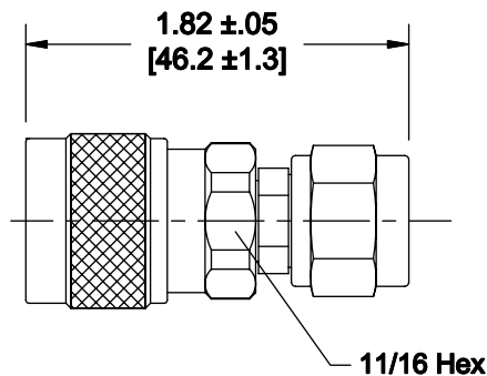
Model Number: 5126 Type N Male / TNC Male
