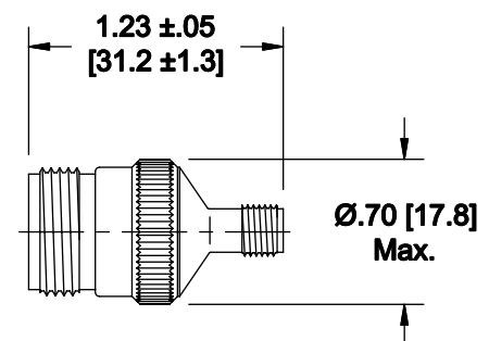
Model Number: 5058 Type N Female / SMA Female
