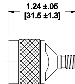
Model Number: 5059 Type N Male / SMA Female
