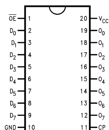
Pin Assignment for DIP and Flatpak
