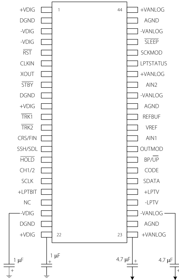
FIGURE 7. BYPASS CIRCUIT
