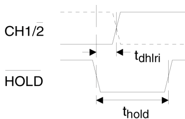
FIGURE 4. START CONVERSION TIMING
