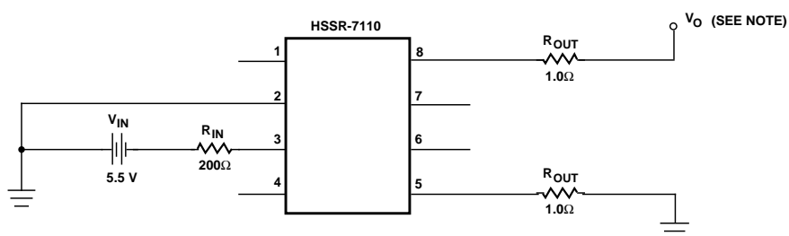
Figure 20. Burn-In Circuit.
