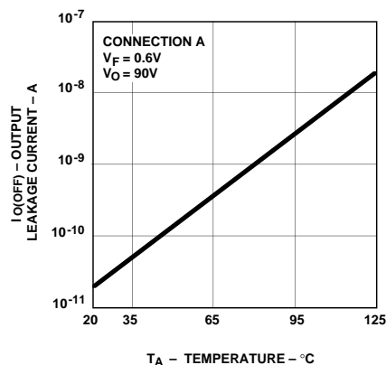
Figure 8. Typical Output Leakage Current vs. Temperature.
