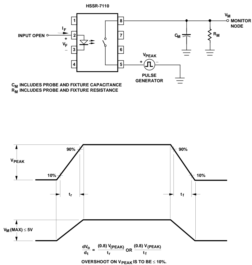
Figure 17. Output Transient Rejection Test Circuit.
