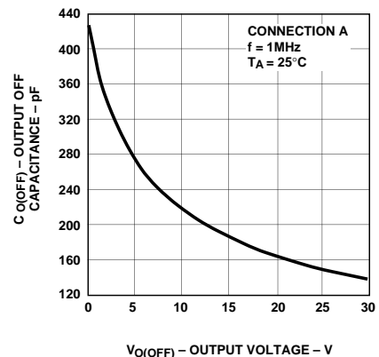
Figure 16. Typical Output Off Capacitance vs. Output Voltage.
