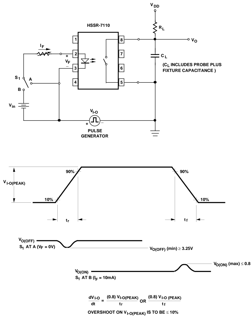
Figure 18. Input-Output Transient Rejection Test Circuit.
