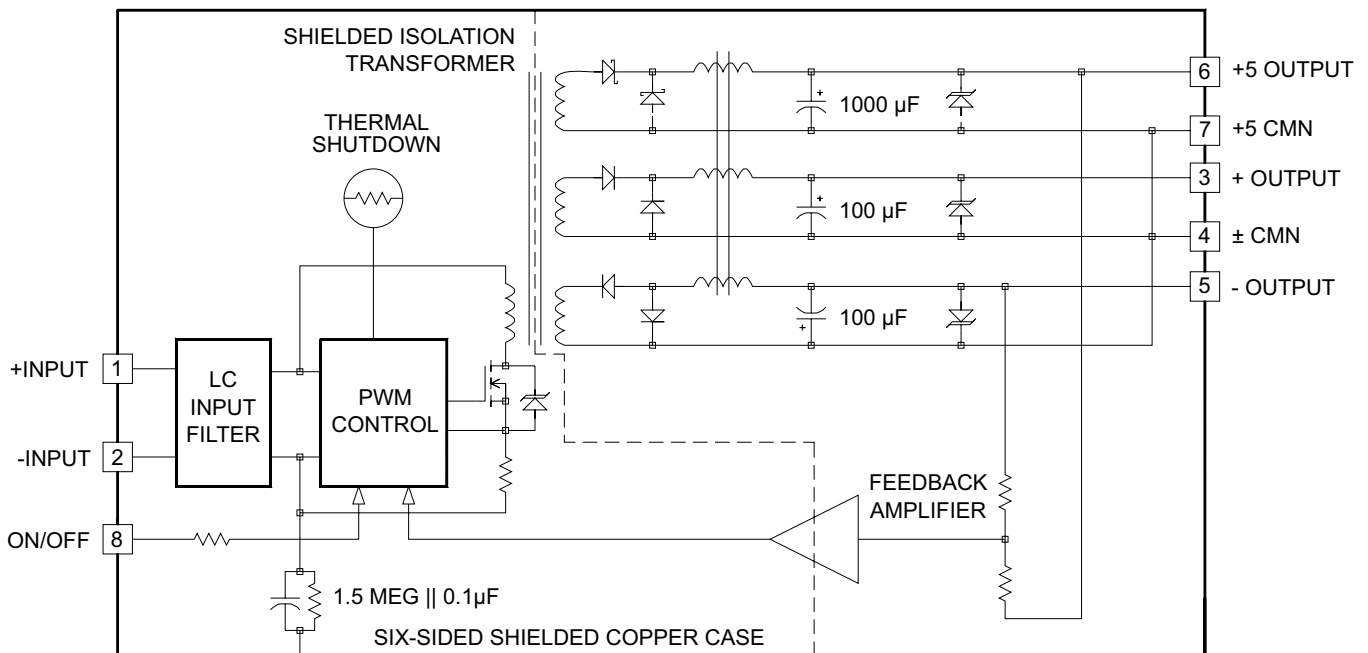
8.5 Watt UW Triple Series Block Diagram
