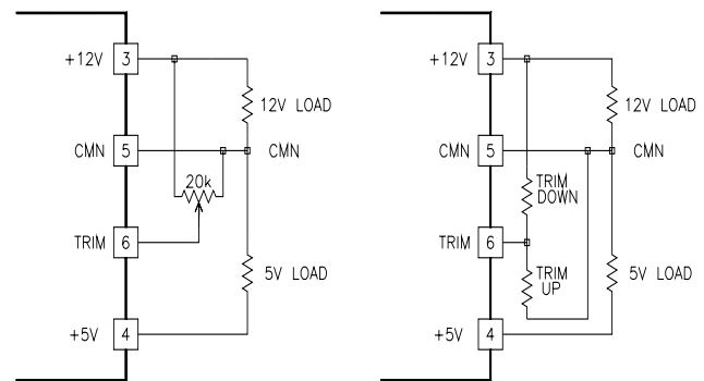
USING TRIMPOT
