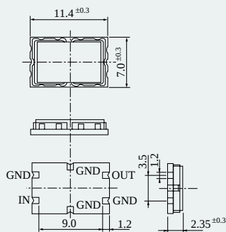
NM1170BA (D-372): Coupling condenser is built-in. (mm)
