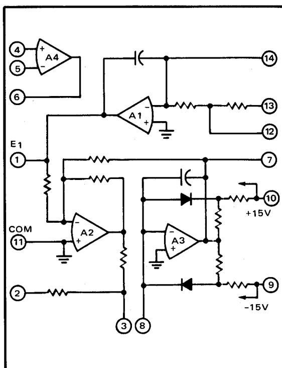
FIGURE 1. Equivalent Circuit.
