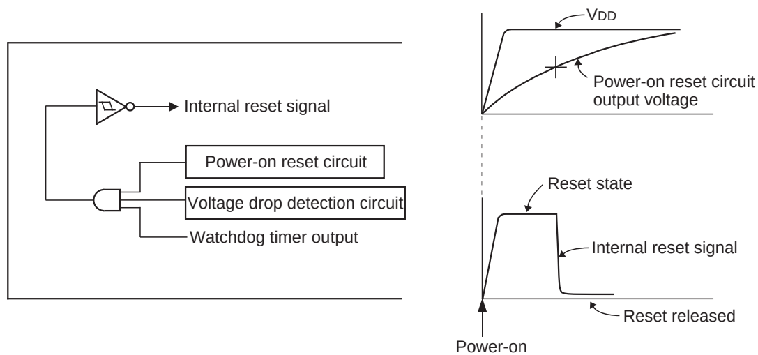
Fig. 18 Power-on reset circuit example
