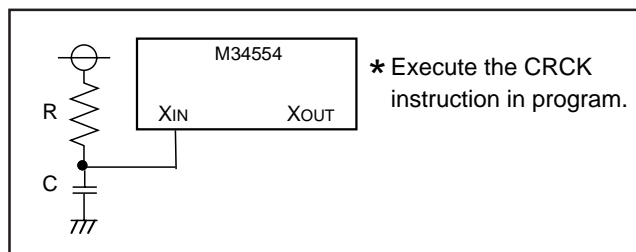
Fig. 50 External RC oscillation circuit
