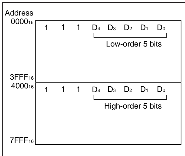
Fig. 60 PROM memory map
