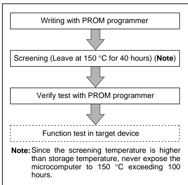
Fig. 61 Flow of writing and test of the product shipped in blank
