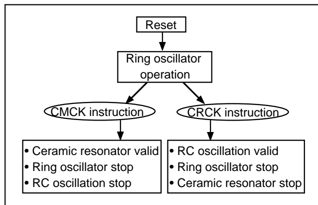
Fig. 47 Switch to ceramic resonance/RC oscillation
