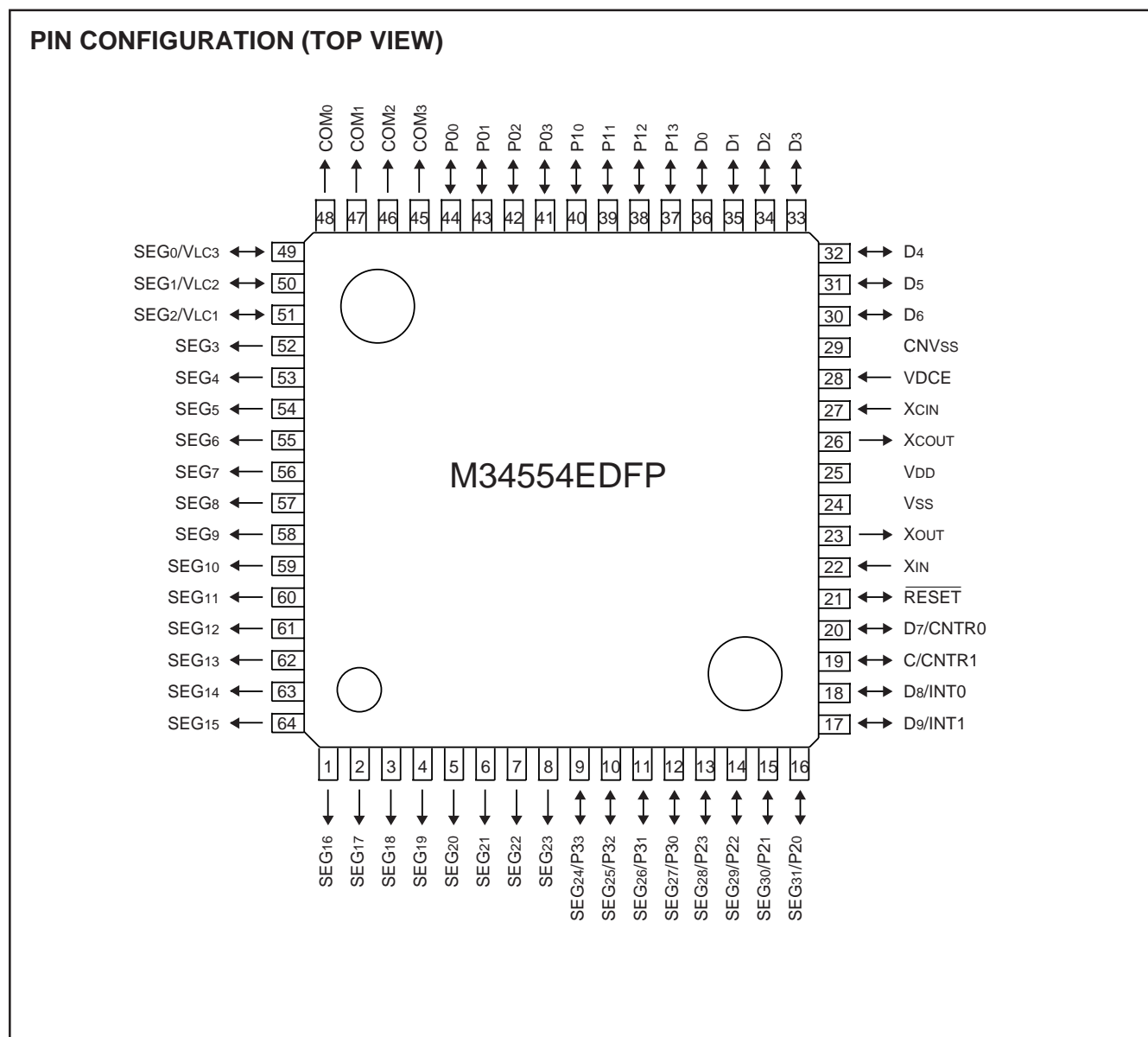
Fig. 59 Pin configuration of built-in PROM version
