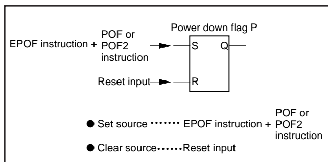
Fig. 44 Set source and clear source of the P flag
