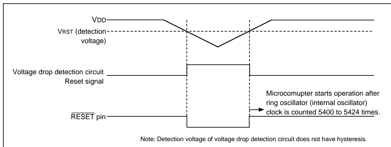
Fig. 42 Voltage drop detection circuit operation waveform
