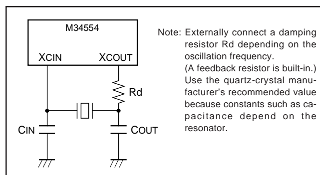
Fig. 52 External quartz-crystal circuit
