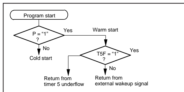
Fig. 45 Start condition identified example using the SNZP instruction
