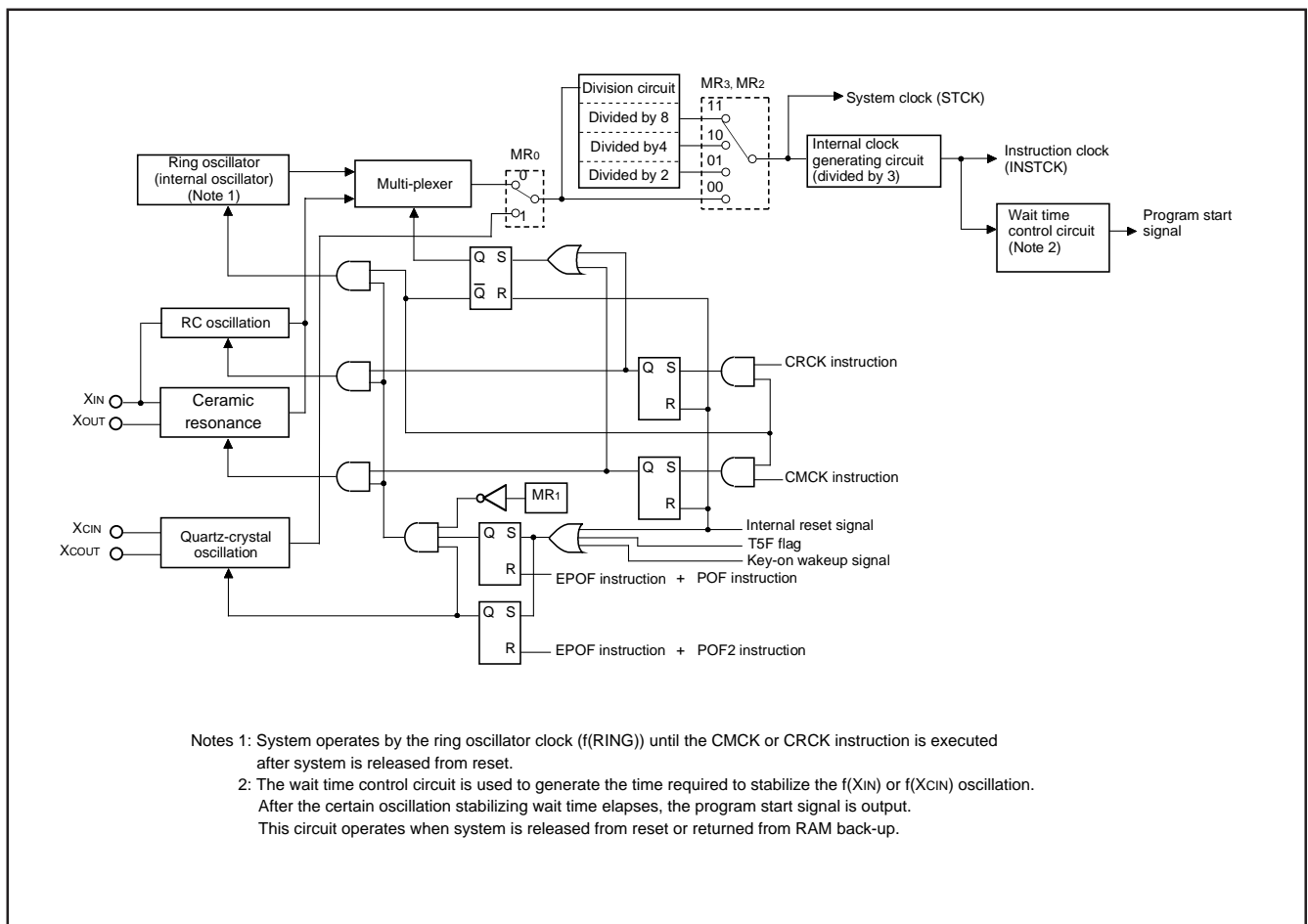
Fig. 46 Clock control circuit structure
