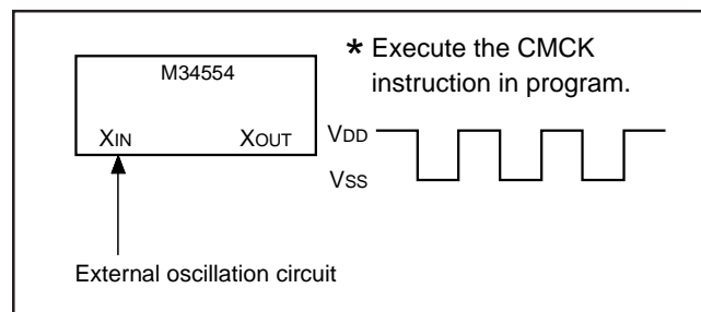
Fig. 51 External clock input circuit
