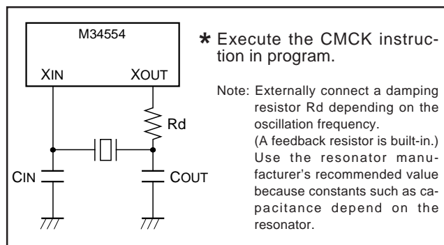
Fig. 49 Ceramic resonator external circuit
