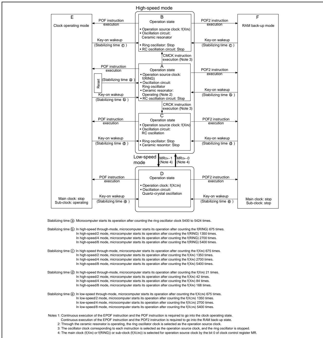
Fig. 43 State transition
