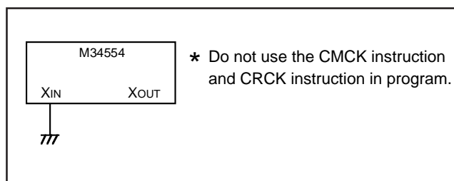
Fig. 48 Handling of X_{IN} and X_{OUT} when operating ring oscillator
