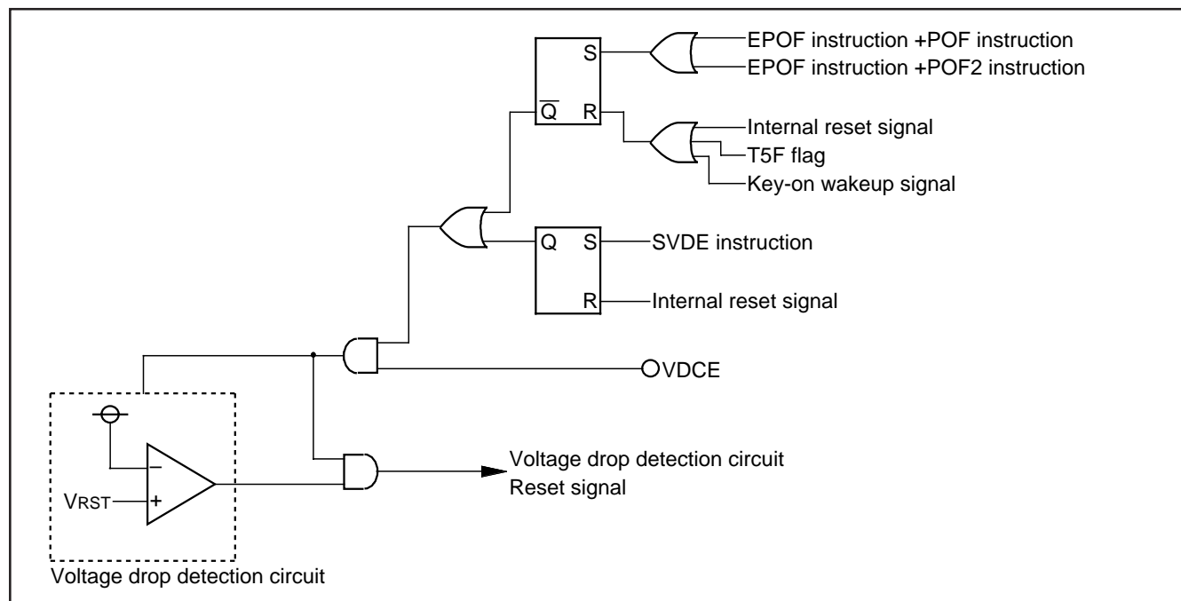
Fig. 41 Voltage drop detection reset circuit
