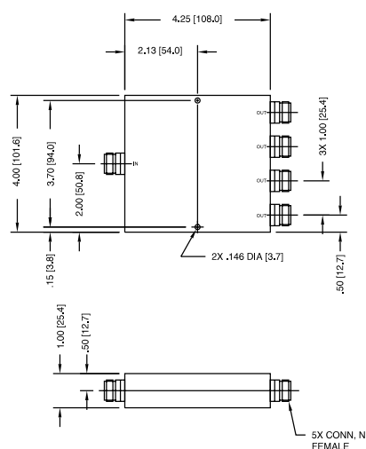
MODEL 3372A-4
