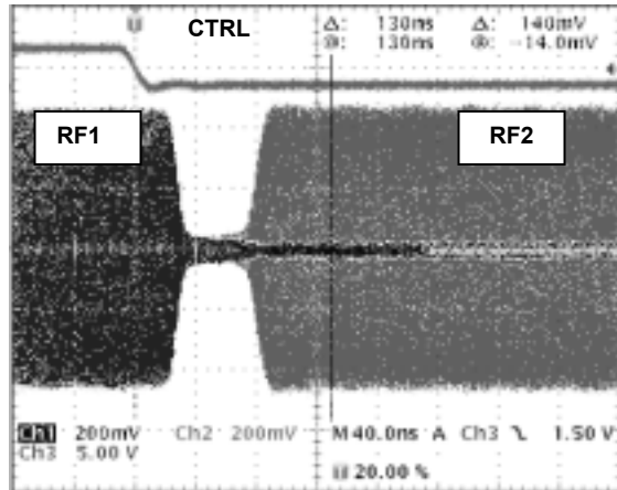
Figure 6. Switching Time
