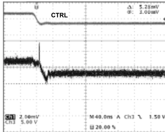
Figure 7. Video Feedthrough*
