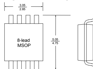
Figure 2. Package Drawings
