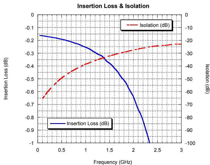
Figure 4. Insertion Loss & Isolation
