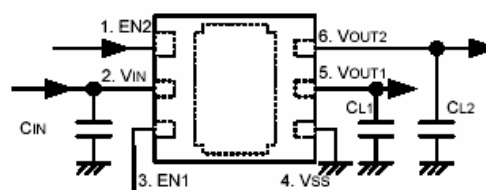
USP-6C (TOP VIEW)
