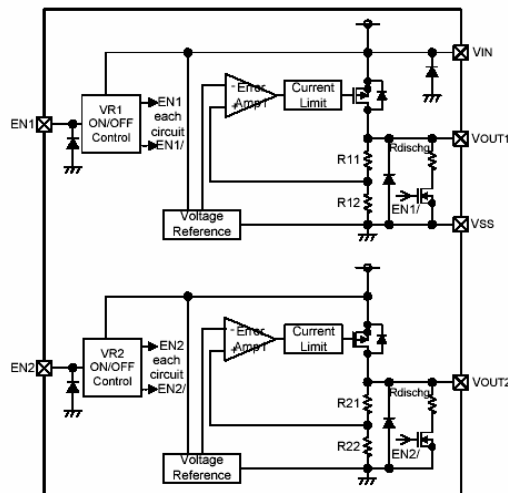
< XC6415BB Series >
