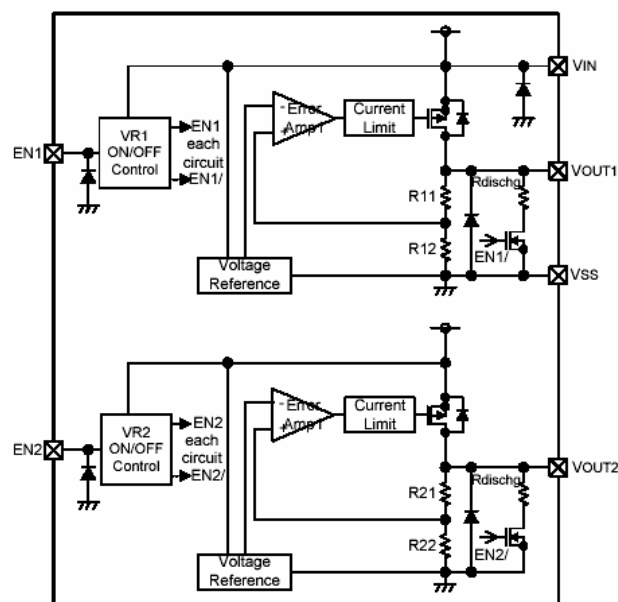
< XC6415BB Series >
