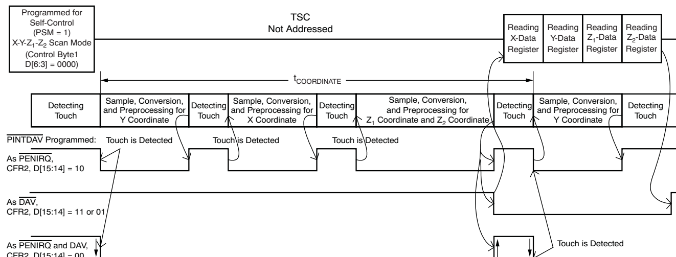
Figure 39. Example of an X, Y, and Z Coordinate Touch Screen Scan using TSMODE 1
