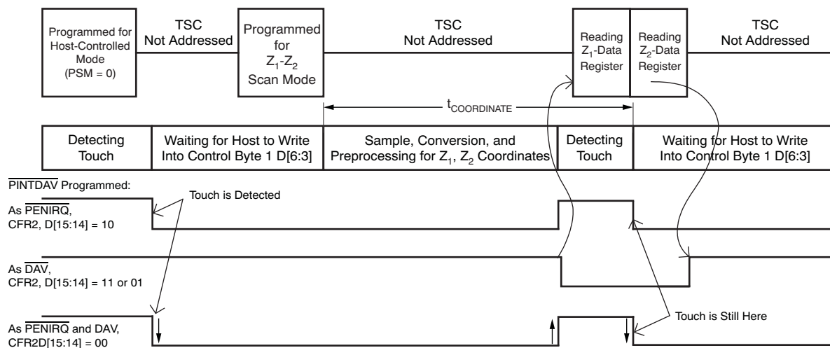
Figure 43. Example of a Z_1 and Z_2 Coordinate Touch Screen Scan (with Panel Stabilization Time) using TSMODE 3
