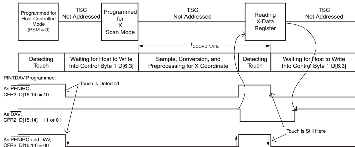
Figure 44. Example of a Single X Coordinate Touch Screen Scan (with Panel Stabilization Time) using TSMODE 3
