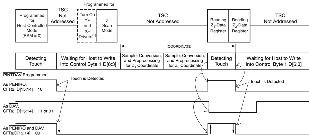
Figure 42. Example of Z_1 and Z_2 Coordinate Touch Screen Scan (without Panel Stabilization Time) using TSMODE 3
