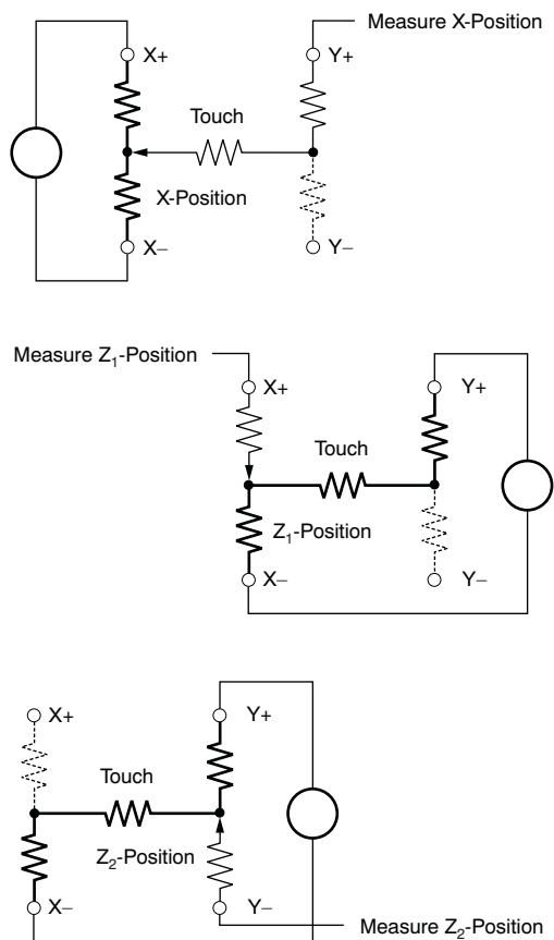
Figure 25. Pressure Measurement
