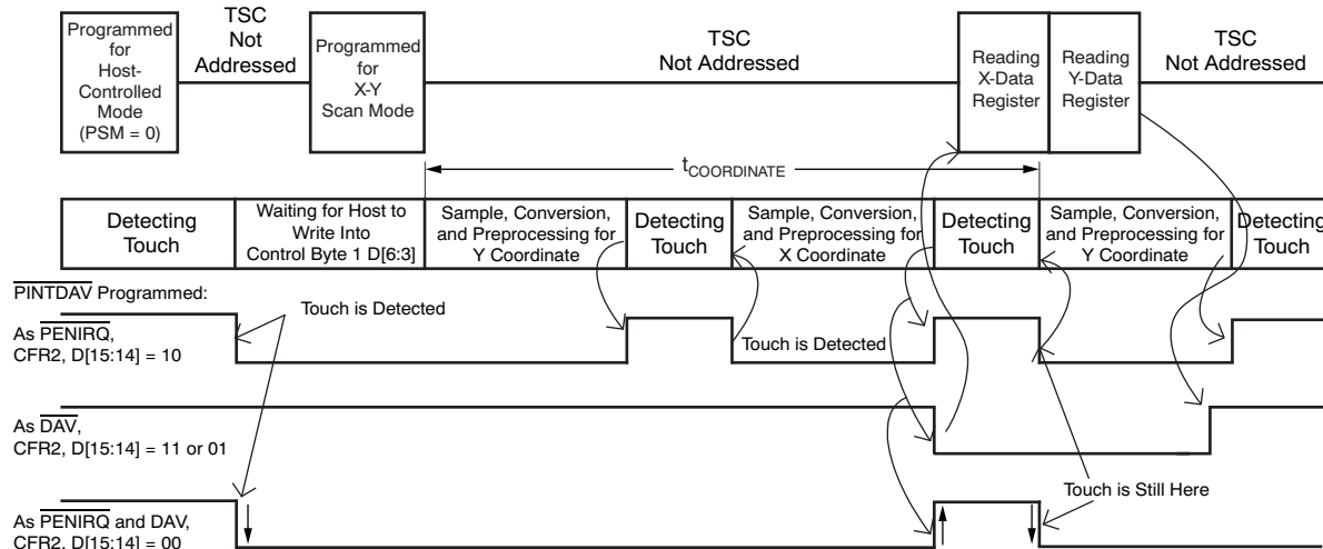
Figure 40. Example of an X and Y Coordinate Touch Screen Scan using TSMODE 2
