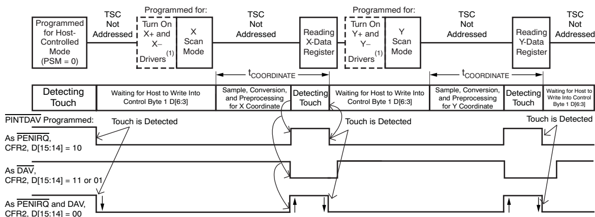
Figure 41. Example of X and Y Coordinate Touch Screen Scan using TSMode 3
