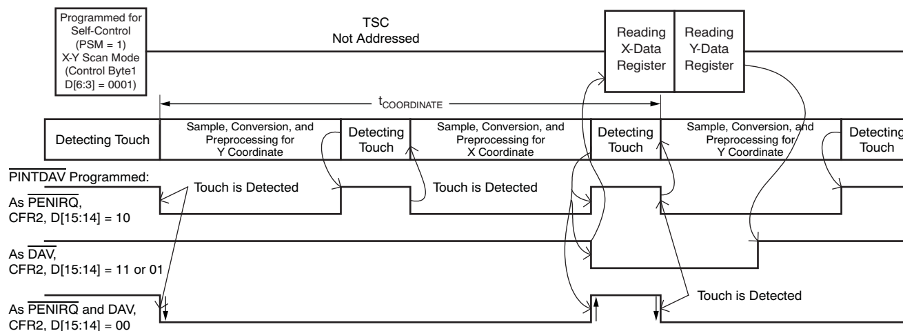
Figure 38. Example of an X and Y Coordinate Touch Screen Scan using TSMODE 1
