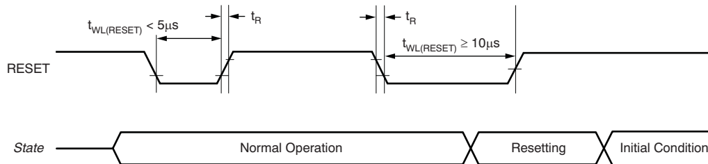
Figure 37. External Reset Timing
