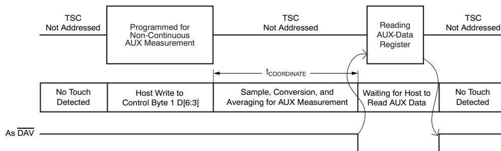
Figure 45. Non-Touch Screen, Non-Continuous AUX Measurement
