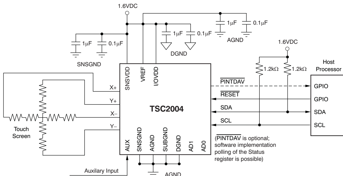
Figure 23. Typical Circuit Configuration
