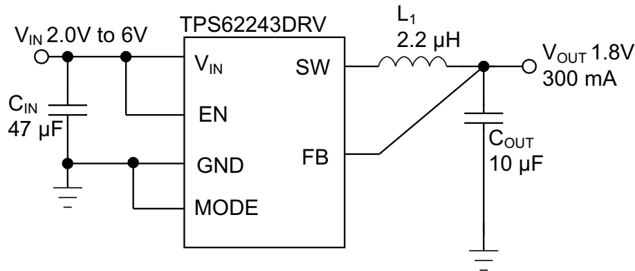
Figure 30. TPS62243 Fixed 1.8 V
