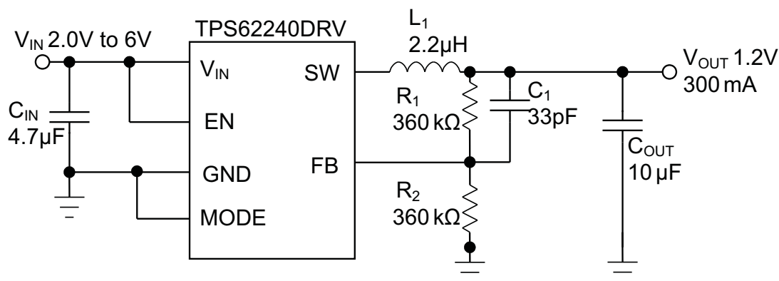
Figure 27. TPS62240DRV Adjustable 1.2 V
