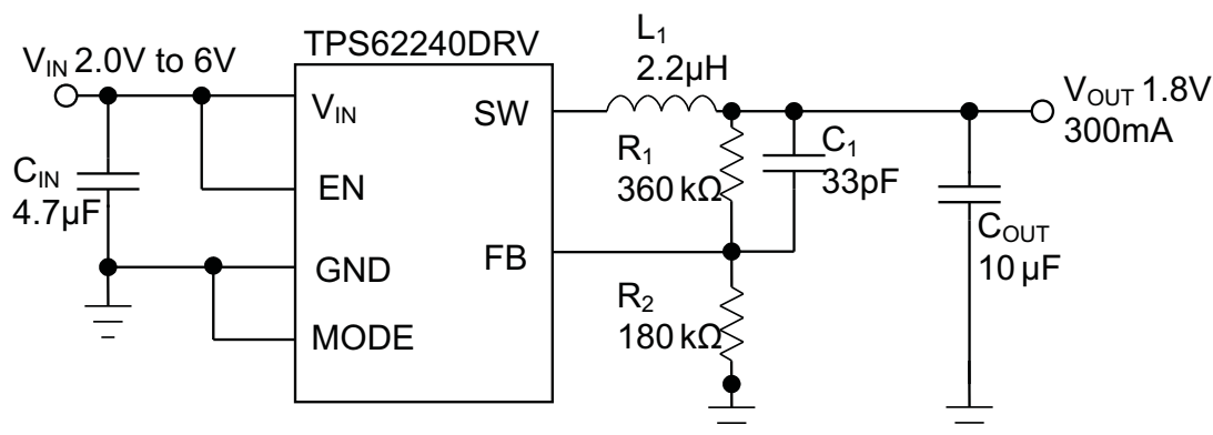
Figure 28. TPS62240DRV 1.8 V
