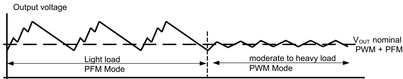
Figure 26. Power Save Mode
