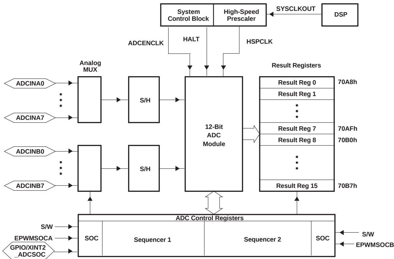
Figure 4-8. Block Diagram of the ADC Module
