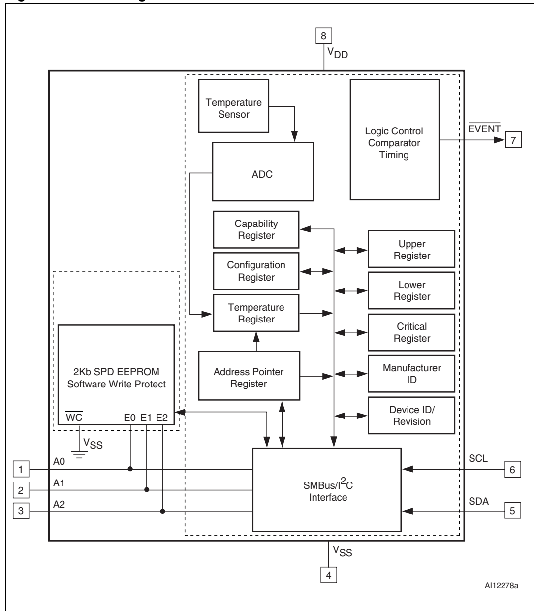
Figure 3. Block diagram
