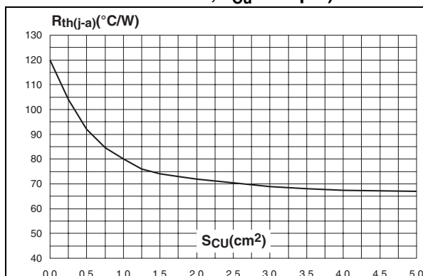
Figure 8. Thermal resistance junction to ambient versus copper surface under each lead (printed circuit board FR4, e_{Cu} = 35 \text{ }\mu\text{m} )
