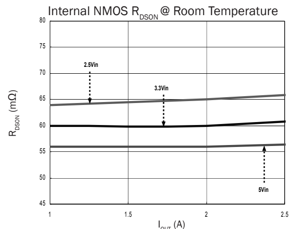
Figure 12. Low-Side N-MOSFET
