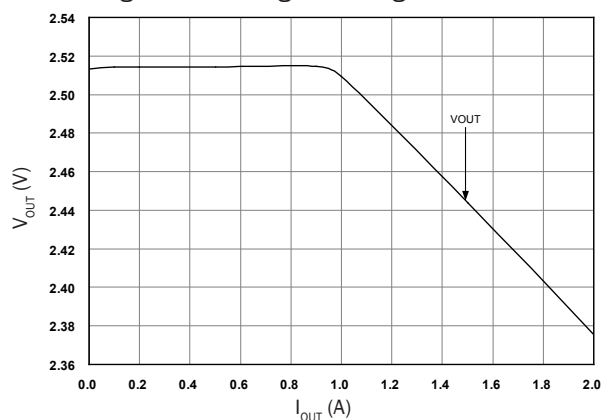
Figure 13. Loading Regulation
