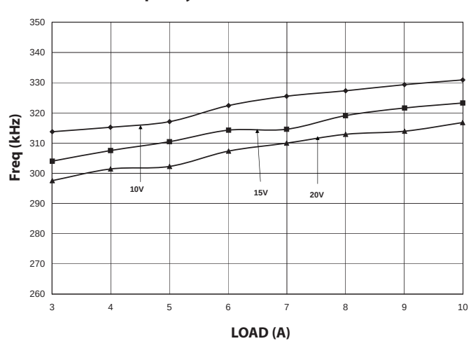
Frequency vs. Load, VOUT1 at 1.8V
