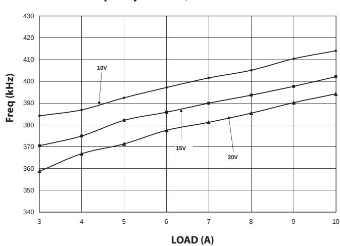
Frequency vs. Load, VOUT2 at 1.5V
