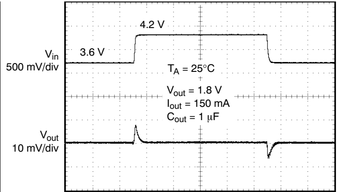
Figure 16. Line Transient
