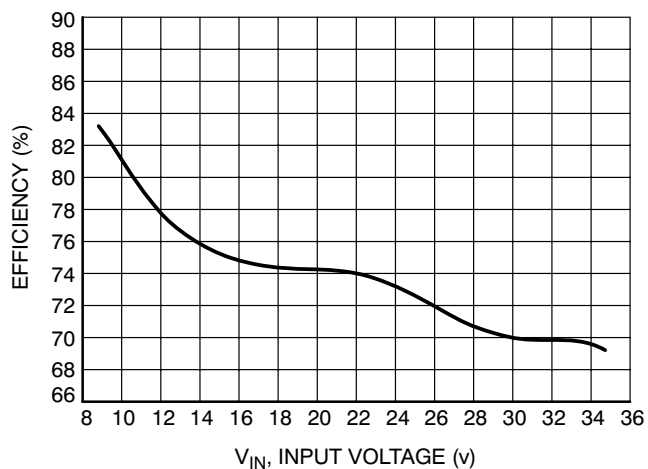
Figure 27. Efficiency vs. Input Voltage for the 3 A Buck Demo Board at I_{OUT} = 3\text{ A} , V_{OUT} = 4\text{ V} , T_A = 25^\circ\text{C}
