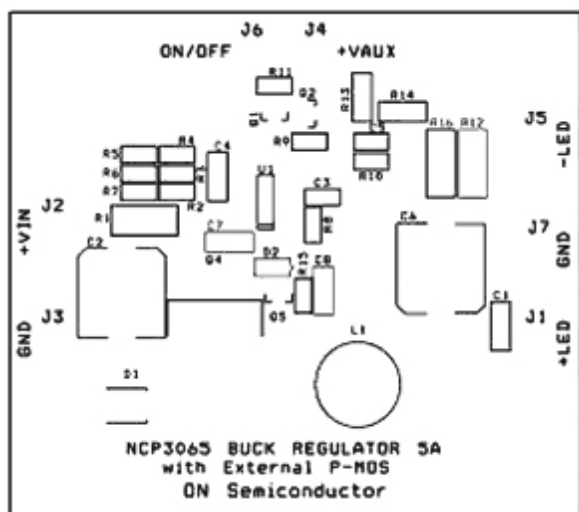
Figure 26. 3 A Buck Demoboard Layout
