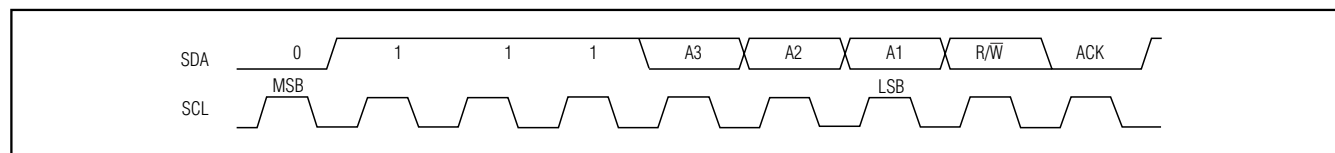
Figure 5. Slave Address
