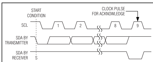
Figure 13. Acknowledge
