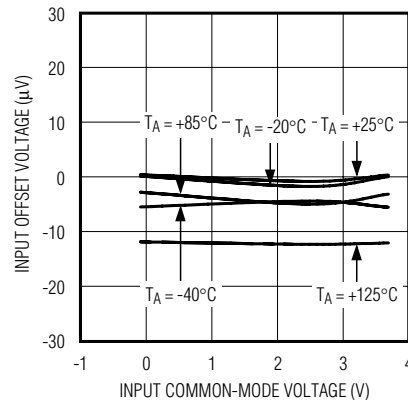
INPUT OFFSET VOLTAGE vs. INPUT COMMON-MODE VOLTAGE
