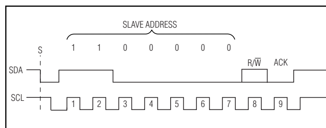
Figure 1. MAX2112 Slave Address Byte
