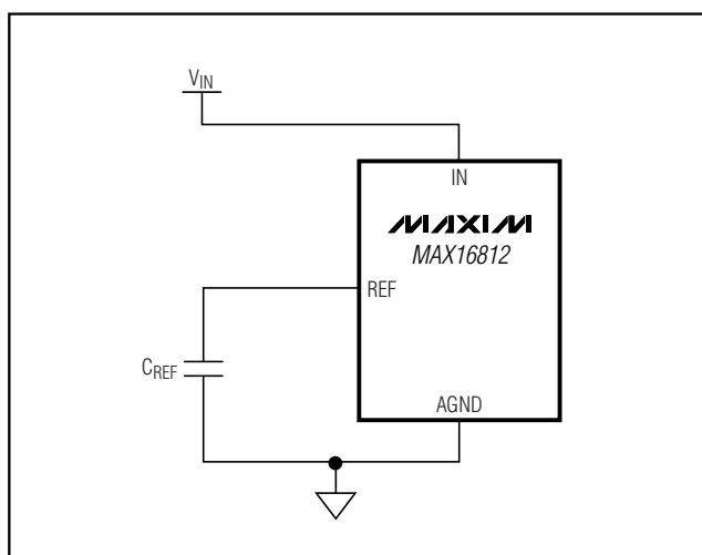
Figure 3. Soft-Start Setting
