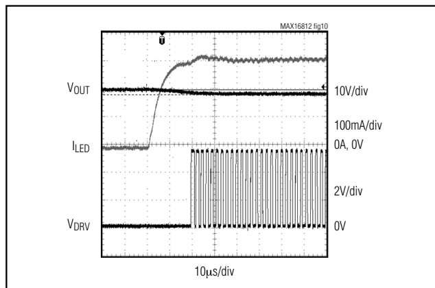
Figure 10. LED Current, Output Voltage, and DRV Waveforms when DIM Signal Goes High
