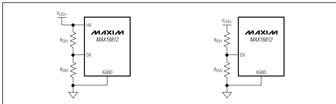
Figure 6. OVP Setting
