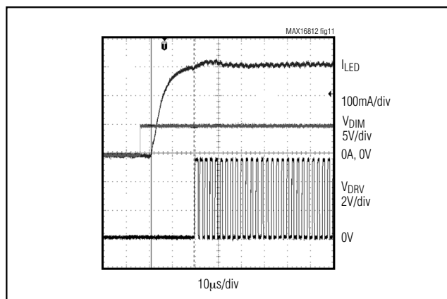
Figure 11. LED Current, DIM Signal, and DRV Waveforms when DIM Signal Goes High
