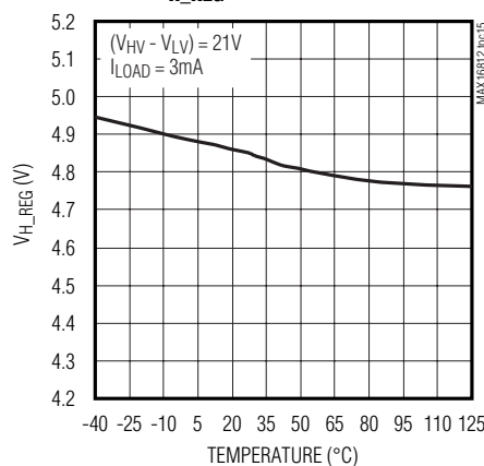
V_{H\_REG} vs. TEMPERATURE
