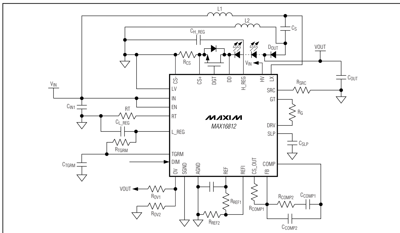
Figure 15. SEPIC Configuration
