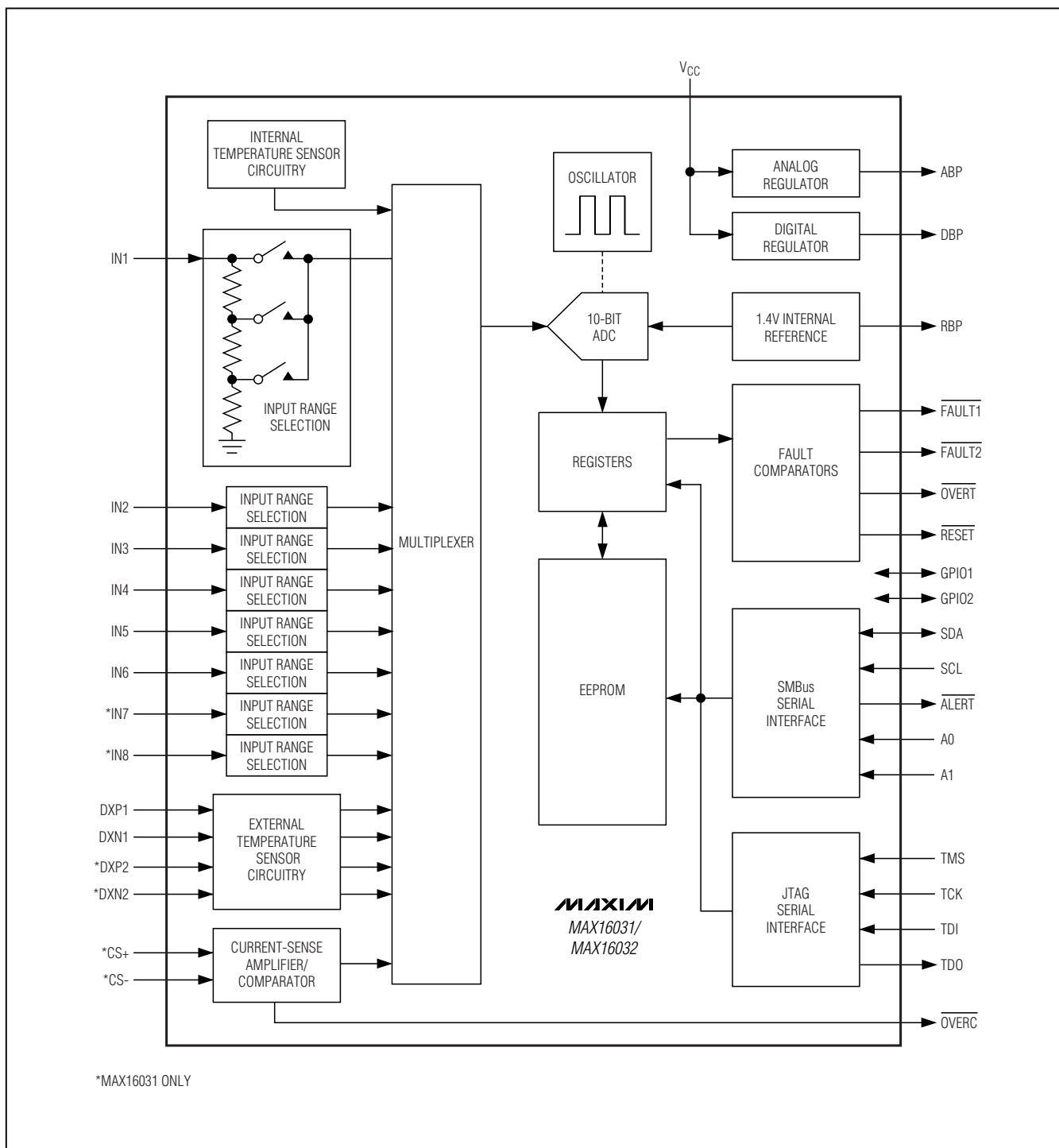
Functional Diagram
