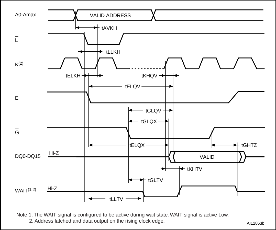
Figure 13. Single synchronous read AC waveforms
