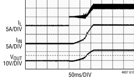
Start-Up with 6V IN to 12V OUT at I OUT = 5A
