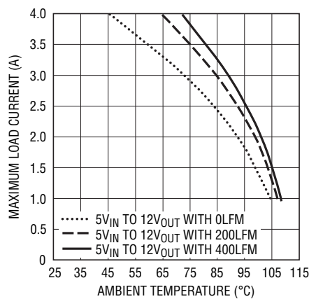
Figure 8. 5V IN to 12V OUT with Heatsink
