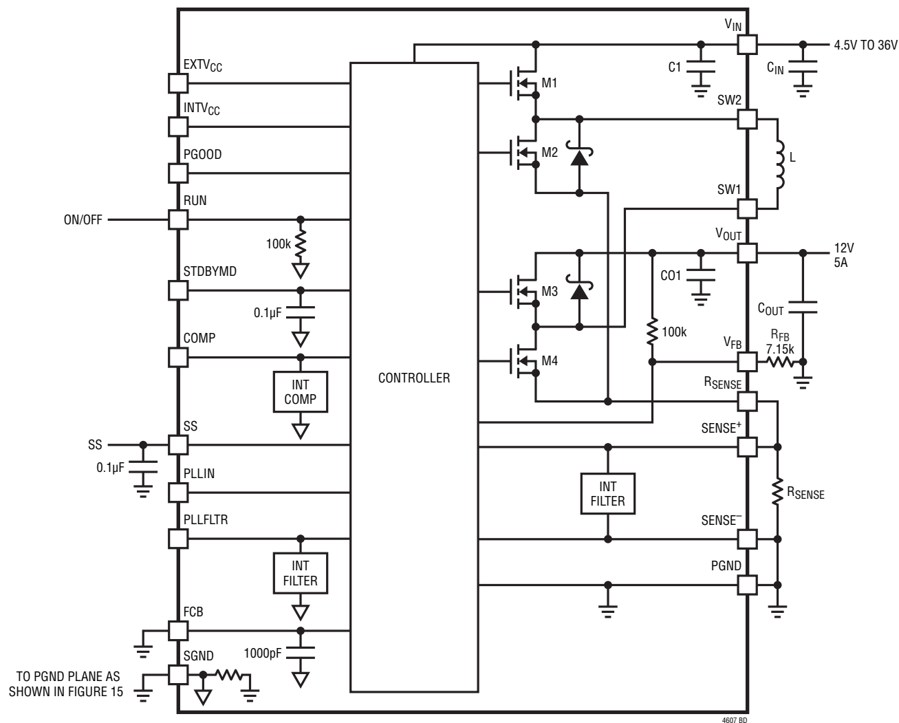
Figure 1. Simplified LTM4607 Block Diagram
