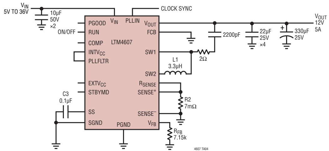
Figure 18. Wide Input Mode with 5V to 36V Input, 12V at 5A Output
