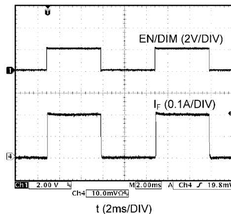
FIGURE 13. PWM Dimming with a 1μF Feed-Forward Capacitor
