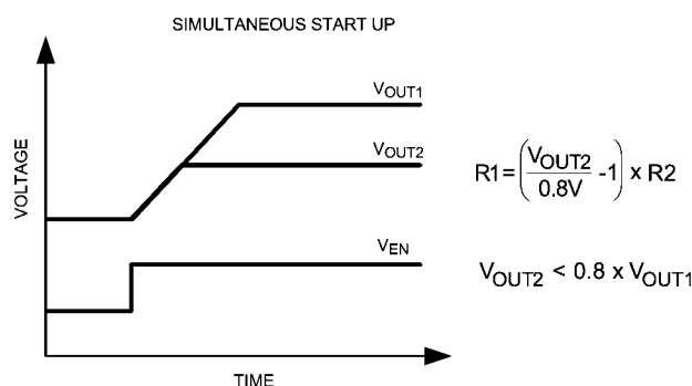
FIGURE 6. Sequencing LM20125 with Precision Enable
