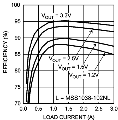
Efficiency vs. Load Current ( V_{IN} = 5\text{V} )
