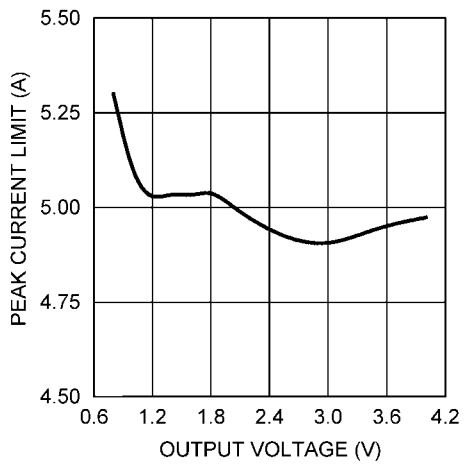
Peak Current Limit vs. V_{\text{OUT}}
