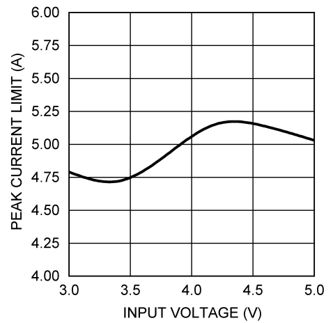
Peak Current Limit vs. V_{\text{IN}}
