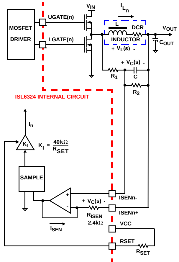
FIGURE 5. INDUCTOR DCR CURRENT SENSING CONFIGURATION
