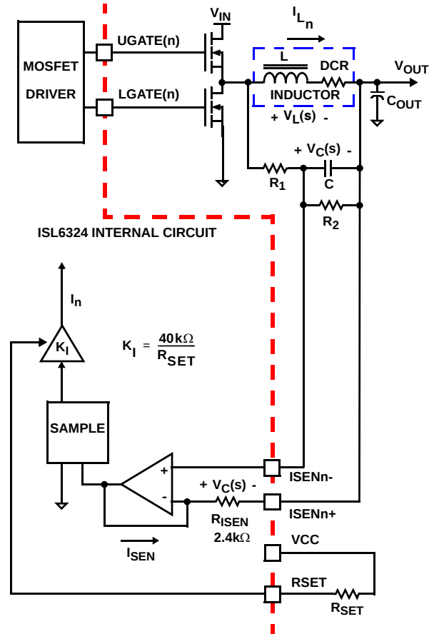
FIGURE 21. DCR SENSING CONFIGURATION
