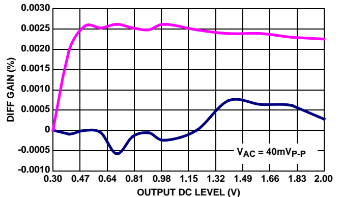
FIGURE 18. DIFFERENTIAL GAIN; f_O = 3.58\text{MHz} , R_L = 150\Omega
