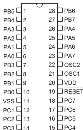
HT82K68E-L/HT82K68A-L —28 SOP-A
